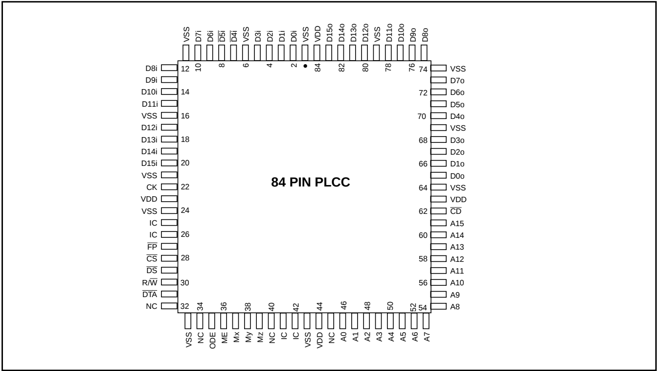
Figure 2 - Pin Connections
