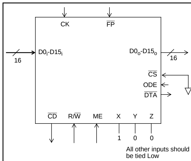
Fig. 10 - Counter Mode Pinout
