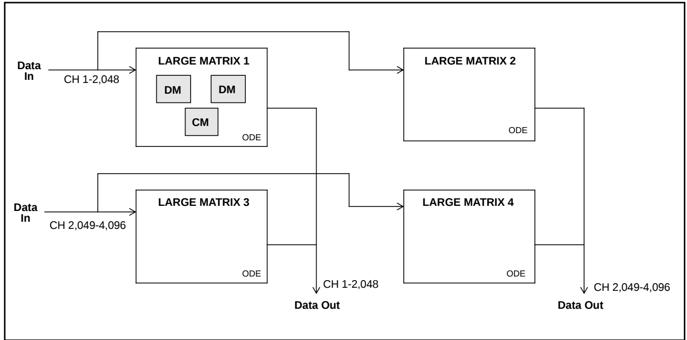
Figure 20 - Extended Switching Matrix
