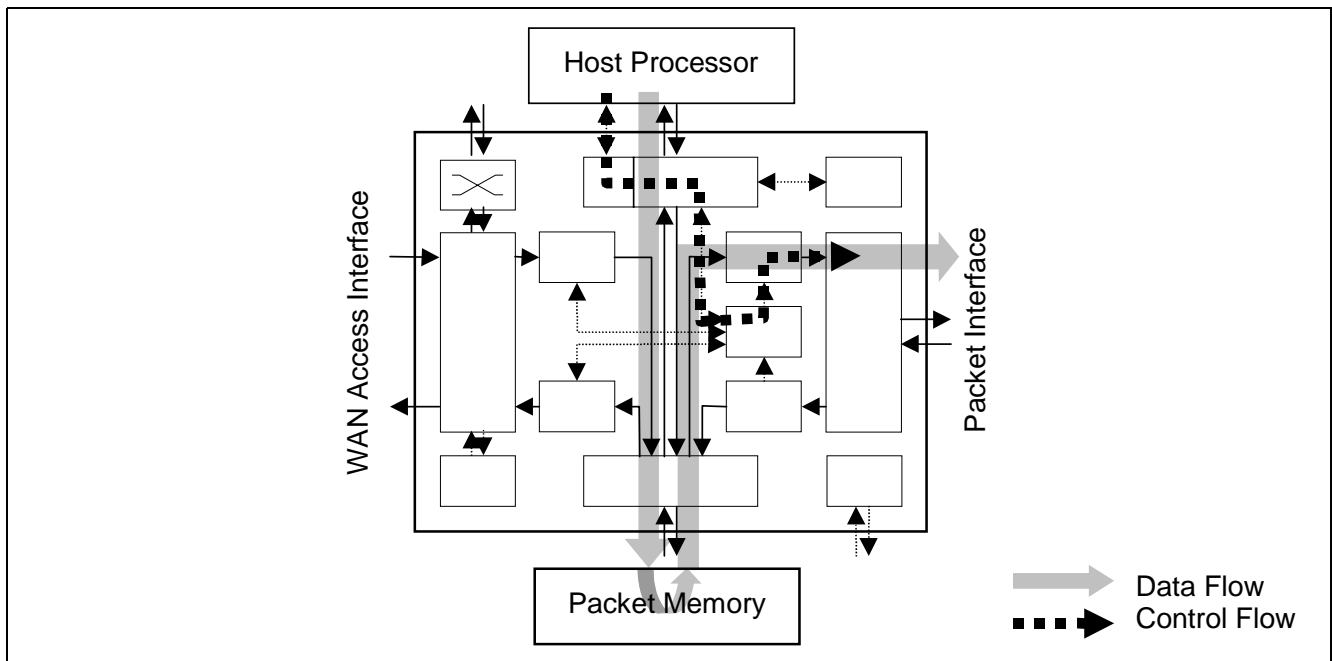
Figure 15 - PCI to Packet Data Flow
