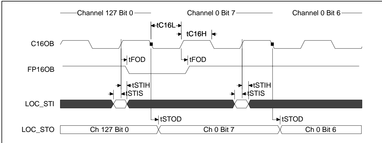
Figure 46 - Local Bus Timing at 8.192 Mbs
