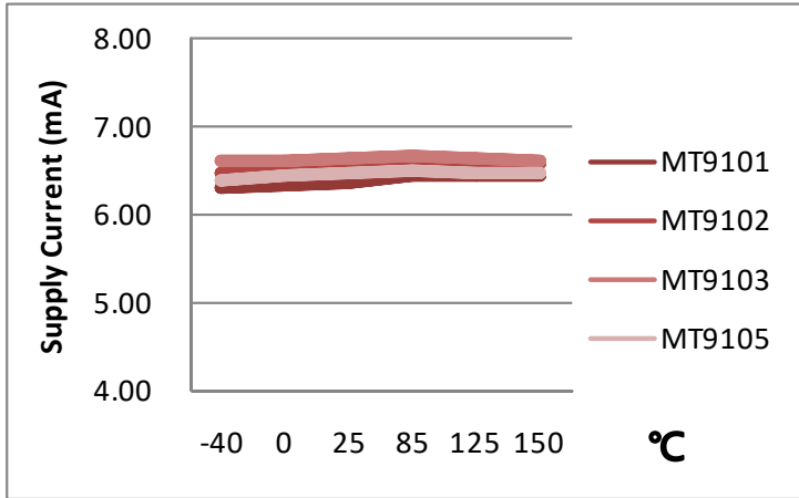
Figure.6 Supply Current vs. Temperature (At Vcc=5.0V)
