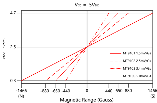
Figure.2 Transfer Characteristics ( V_{CC}=5V )
