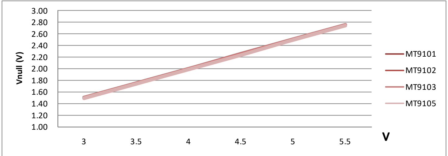
Figure.12 V_{NULL} vs. V_{CC} (At B=0Gs ; T_A=25^{\circ}C )
