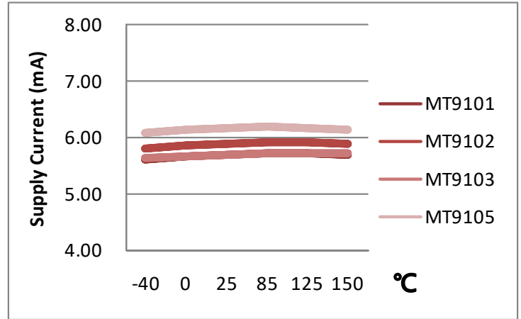
Figure.7 Supply Current vs. Temperature (At Vcc=3.3V)
