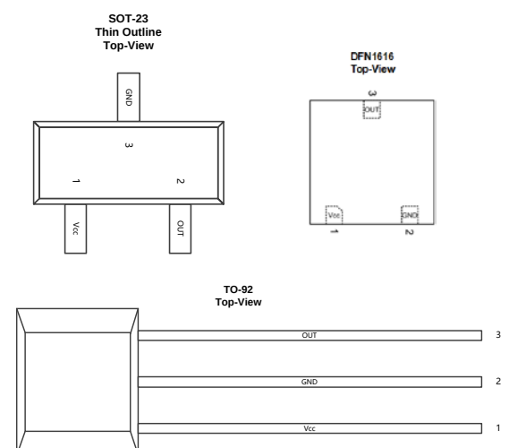
Figure.1 Pin Configuration & Functions
