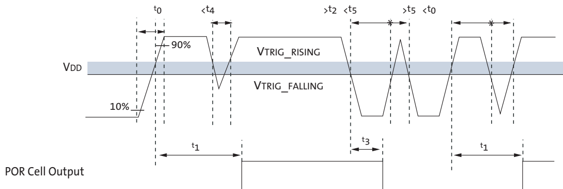
Figure 27: Internal Power-On Reset
