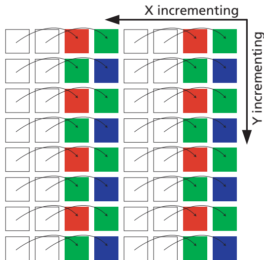
Figure 15: Pixel Readout ( x\_odd\_inc=3 , y\_odd\_inc=1 , x\_bin=1 )
