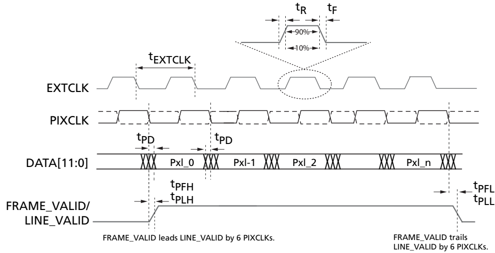
Figure 36: I/O Timing
