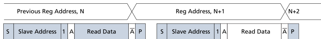
Figure 25: Single Read from Current Location
