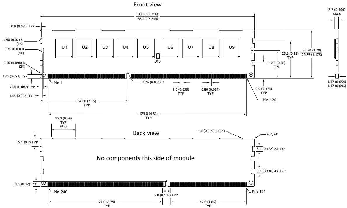
Figure 4: 240-Pin DDR3 UDIMM (PCB 1125)
