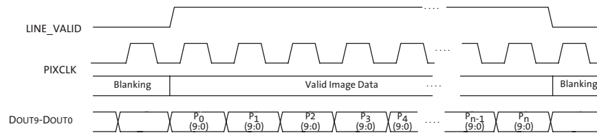
Figure 7: Timing Example of Pixel Data
