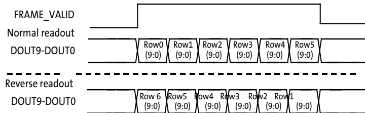
Figure 16: Readout of 6 Rows in Normal and Row Mirror Output Mode
