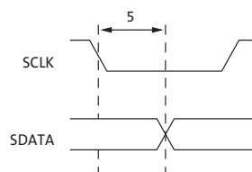
Figure 25: Serial Host Interface Data Timing for Read
