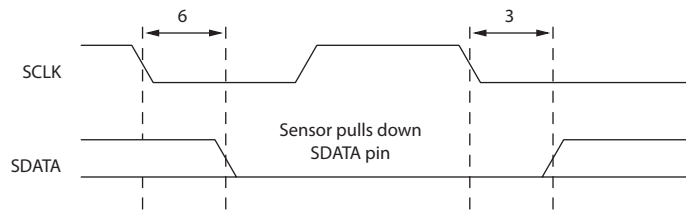
Figure 26: Acknowledge Signal Timing After an 8-bit Write to the Sensor
