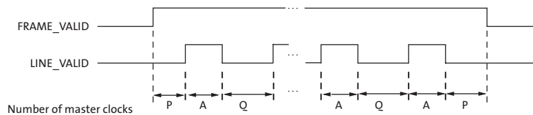
Figure 8: Row Timing and FRAME_VALID/LINE_VALID Signals
