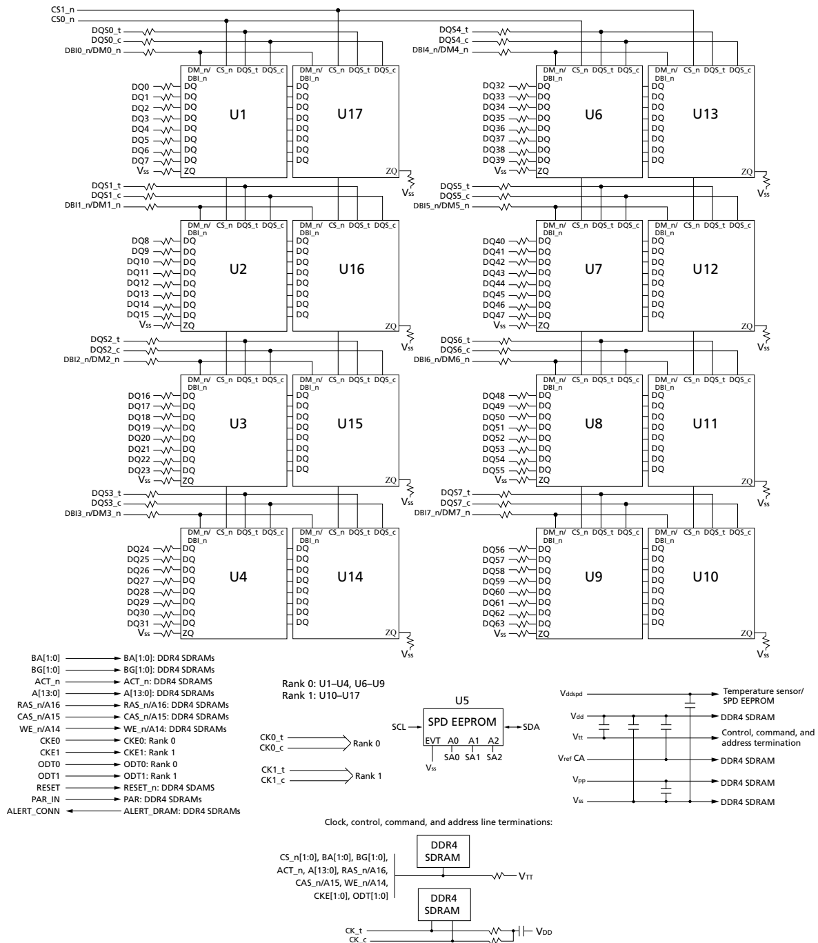
Figure 3: Functional Block Diagram (R/C-B1 PCB 1866)
