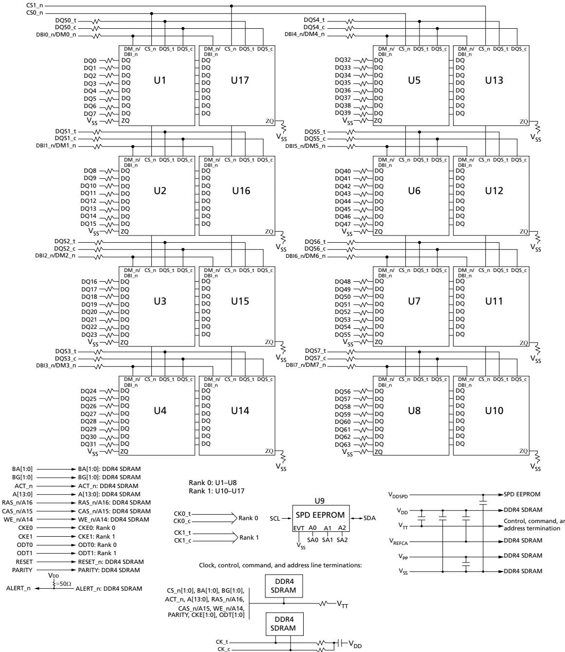
Figure 2: Functional Block Diagram (R/C-B PCB 1447)
