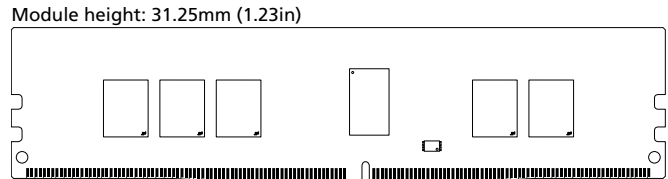
Figure 1: 288-Pin RDIMM (MO-309, R/C-D)
