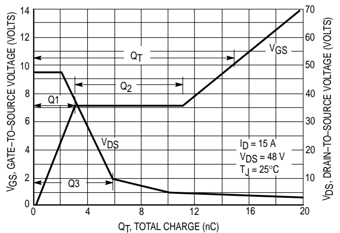
Figure 6. Gate-to-Source and Drain-to-Source Voltage versus Total Charge
