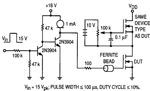
Figure 5. Gate Charge Test Circuit
