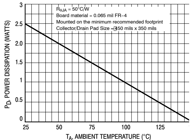
Figure 15. D²PAK Power Derating Curve
