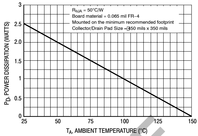
Figure 15. D²PAK Power Derating Curve
