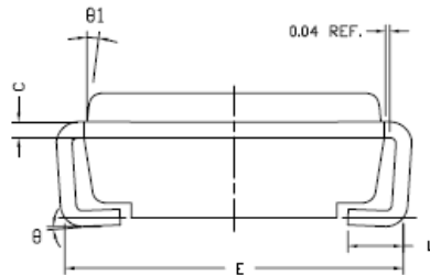
8-Lead 2928-8J Plastic Package CYStek Package Code: N8J
