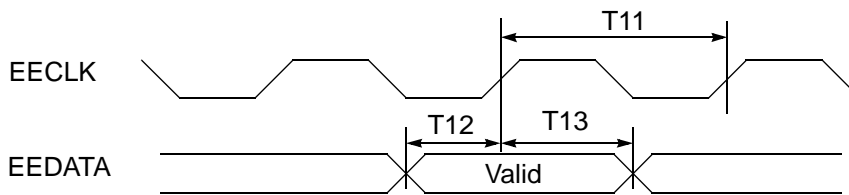
FIGURE 4. EEPROM timing
