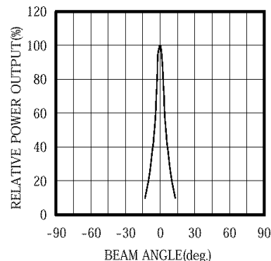
RADIATION PATTERN
