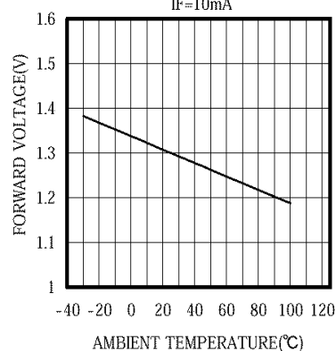
FORWARD VOLTAGE vs TEMPERATURE IF=10mA
