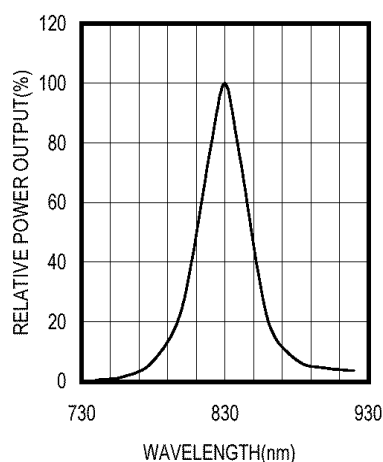
SPECTRAL OUTPUT
