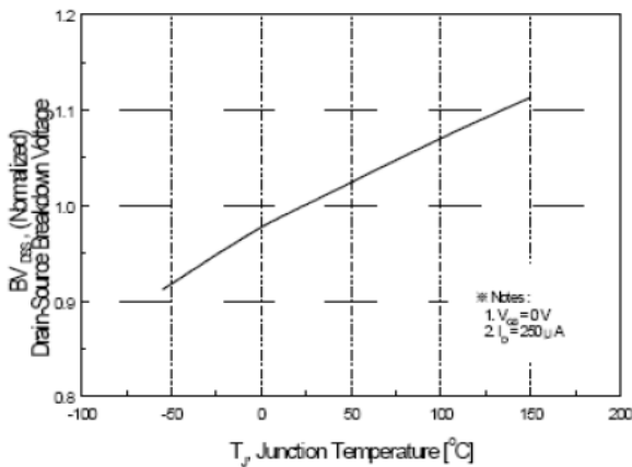
Figure 8. Breakdown Voltage Variation vs Temperature
