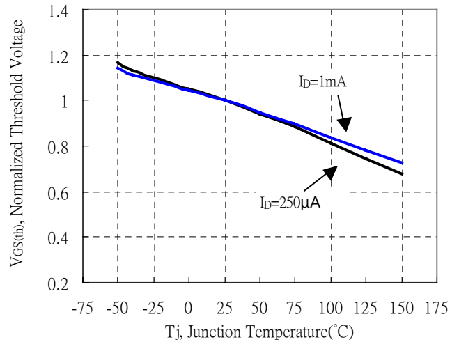
Threshold Voltage vs Junction Teaperture
