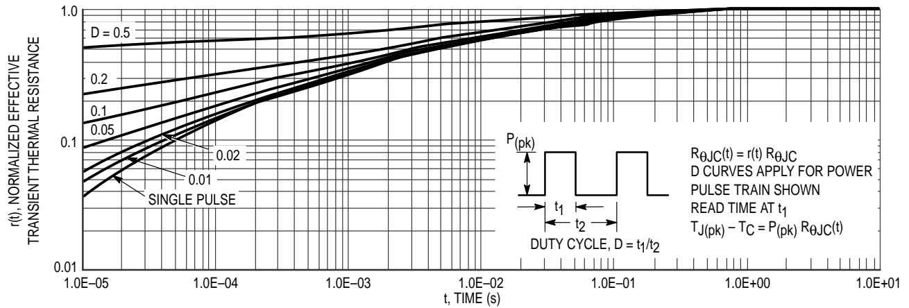
Figure 14. Thermal Response
