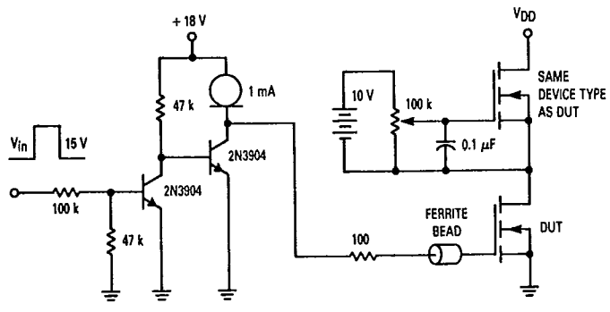
Figure 18. Gate Charge Test Circuit
