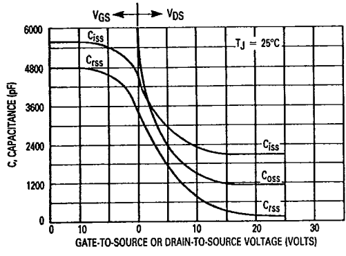
Figure 16. Capacitance Variation
