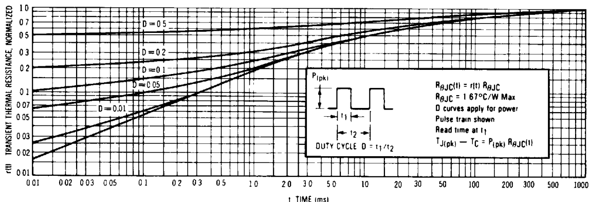
Figure 10. Thermal Response
