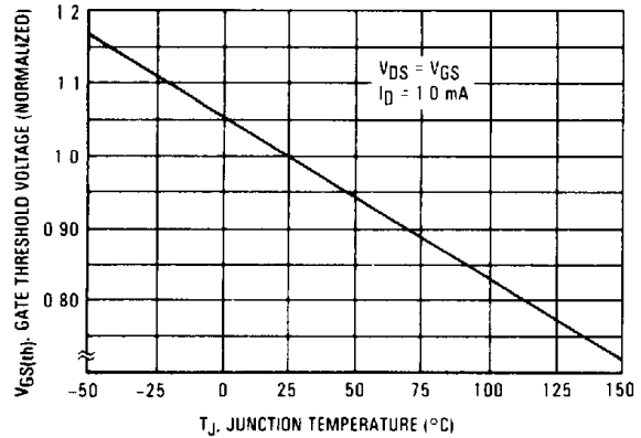
Figure 2. Gate-Threshold Voltage Variation With Temperature
