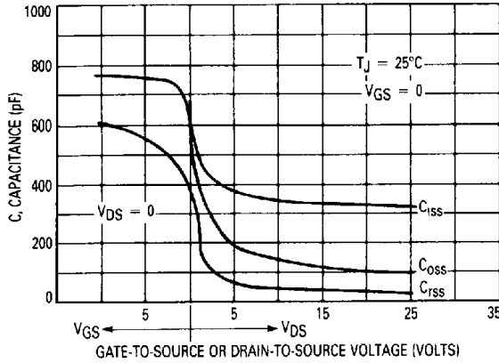
Figure 11. Capacitance Variation
