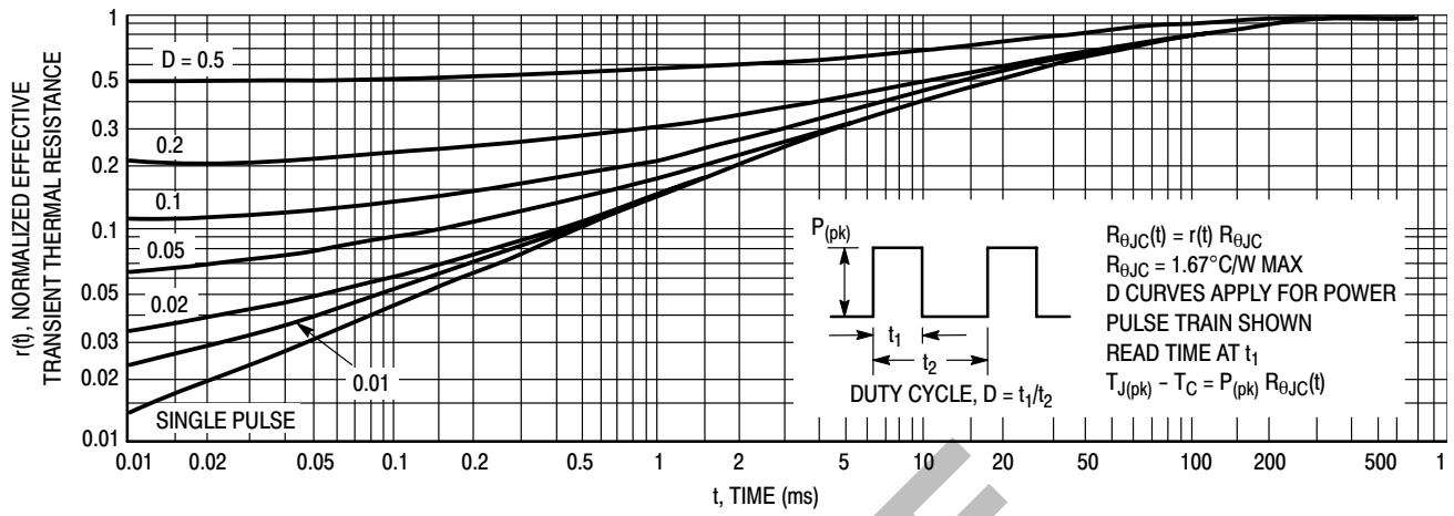
Figure 10. Thermal Response
