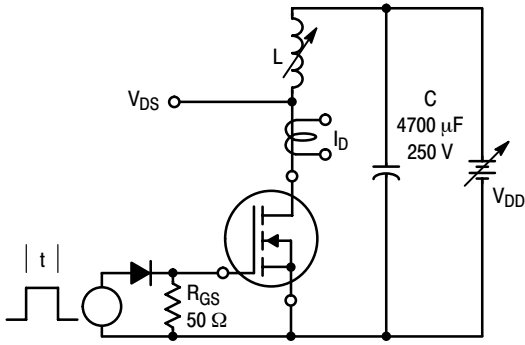
Figure 16. Unclamped Inductive Switching Test Circuit
