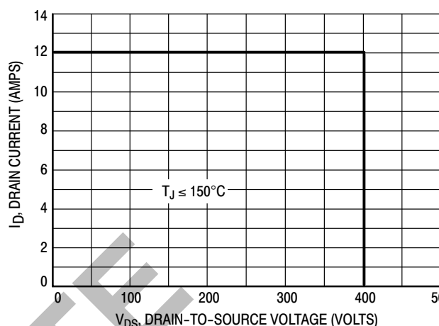
Figure 8. Maximum Rated Switching Safe Operating Area
