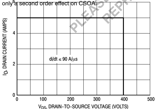
Figure 13. Commutating Safe Operating Area (CSOA)
