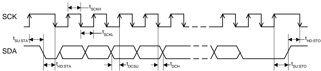
FIGURE 12. Data Interface Timing(I 2 C)
