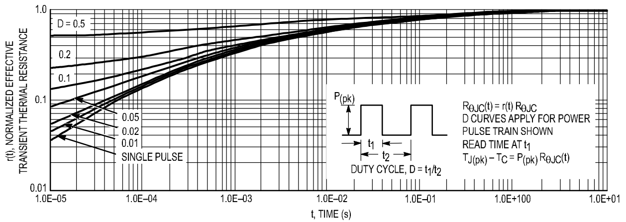
Figure 13. Thermal Response
