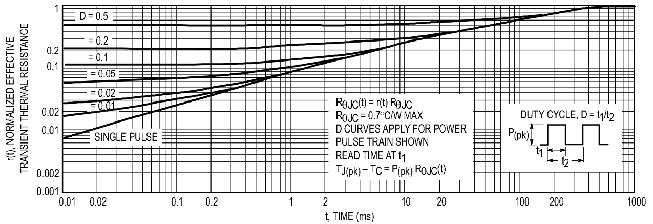
Figure 13. Thermal Response
