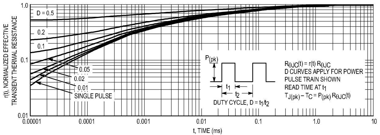
Figure 13. Thermal Response
