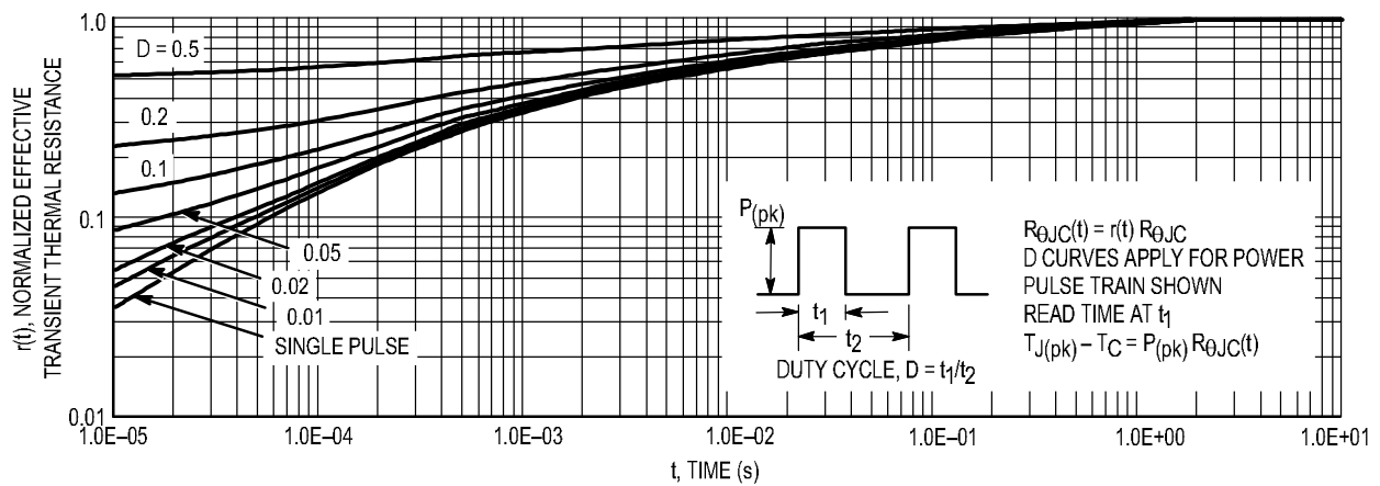
Figure 13. Thermal Response
