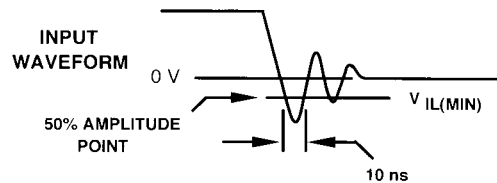
Figure 9: V IL Waveform
