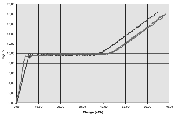
Typ. gate charge
