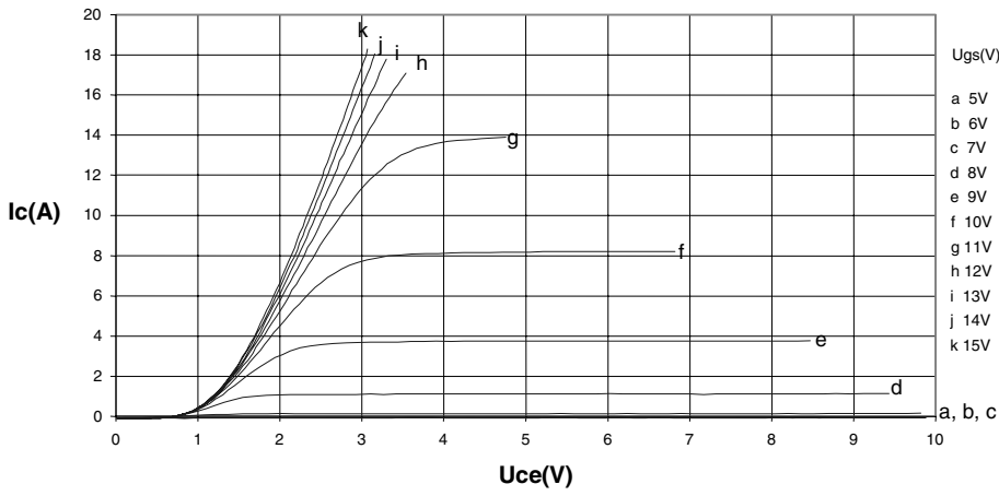
Typ. output characteristics 25°C
