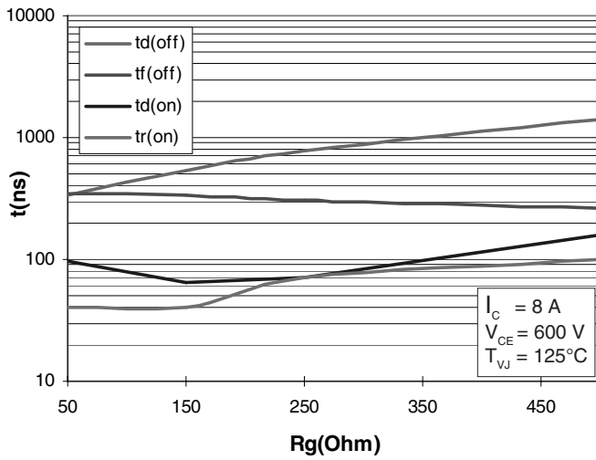
Typ. switching time
