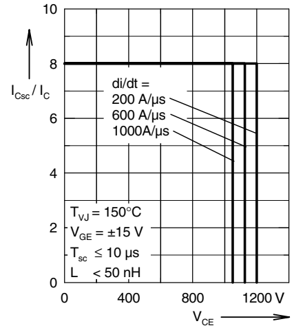
Short circuit safe operating area
