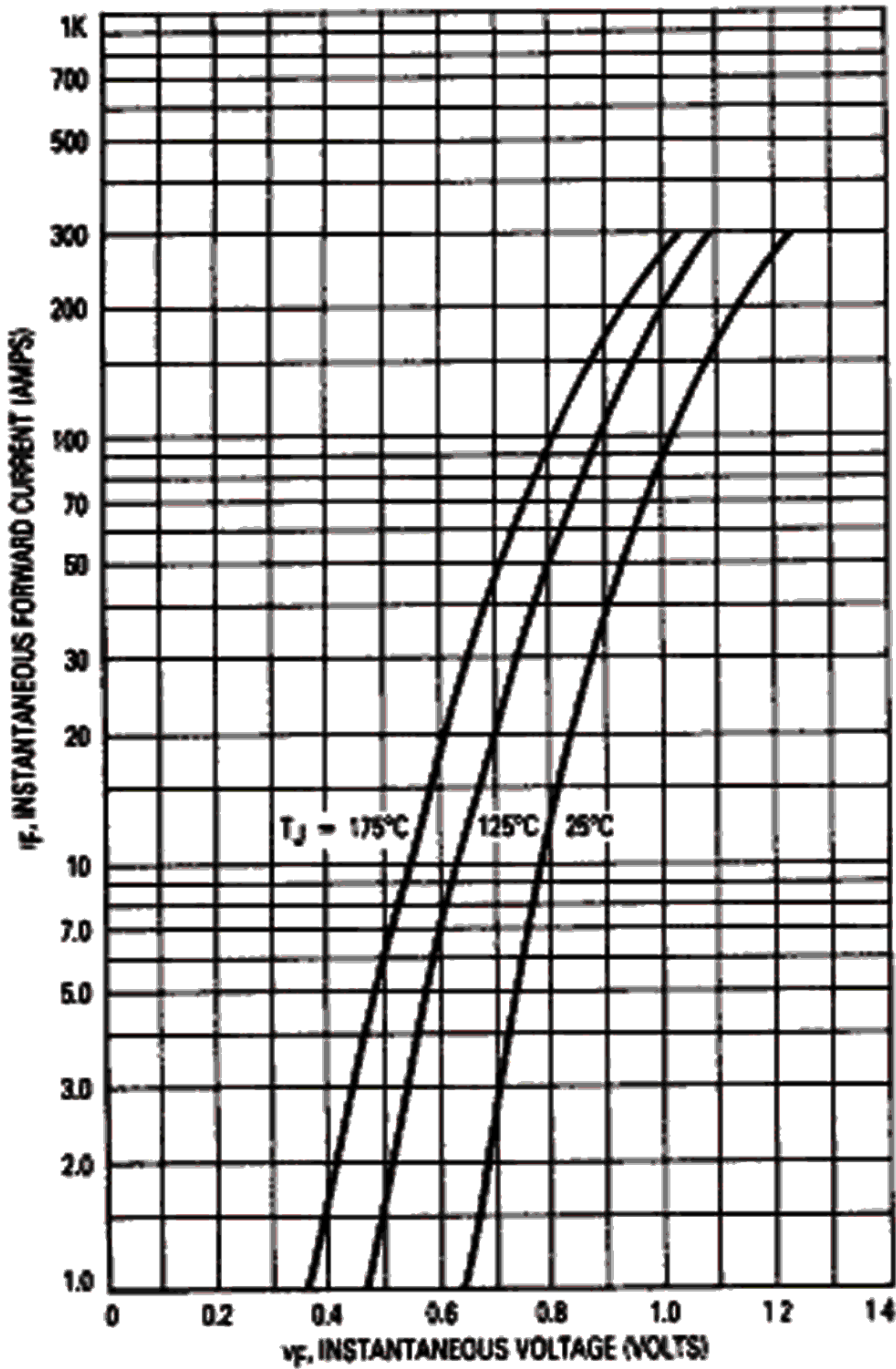
FIGURE 1 — FORWARD VOLTAGE
