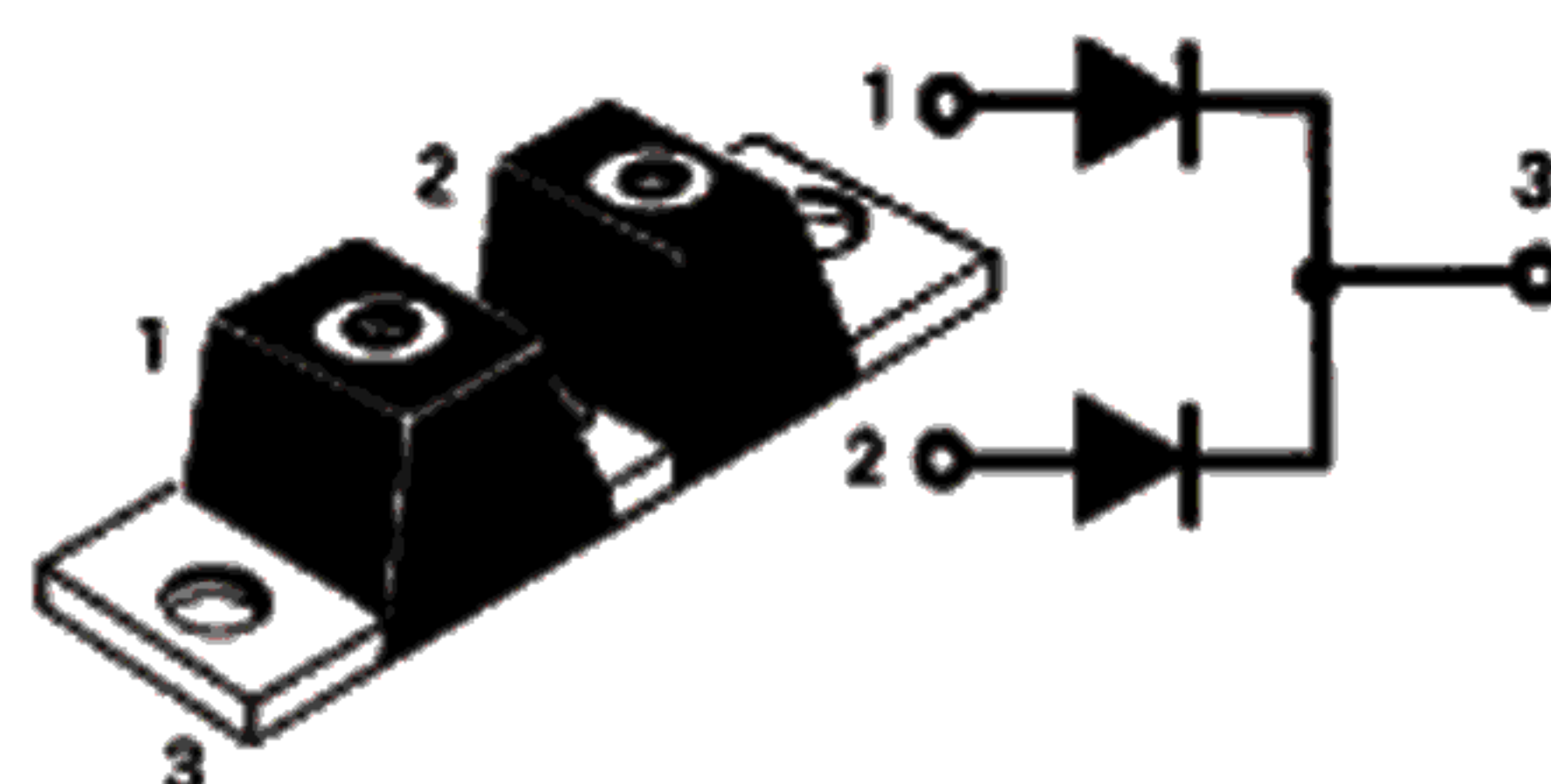
CASE 357C-03
