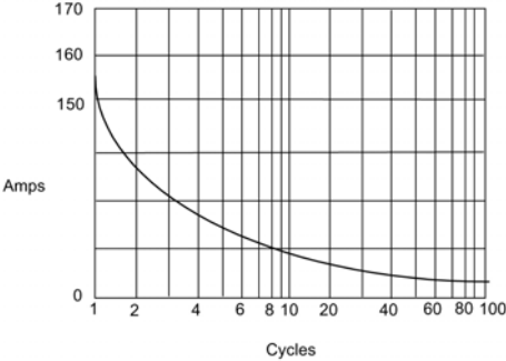
Figure 4 Maximum Non-Repetitive Forward Surge Current
