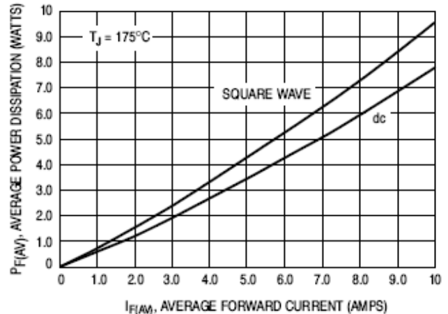
Figure 5. Power Dissipation
