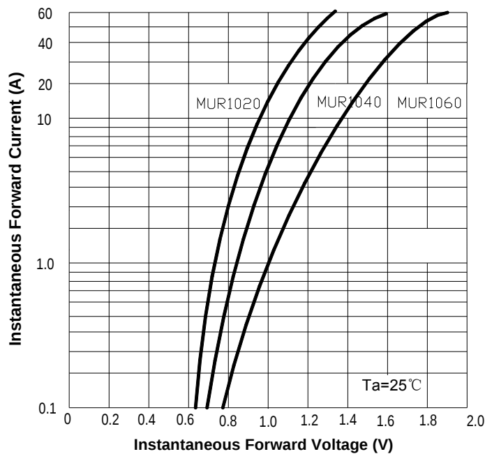
FIG3: Forward Voltage
