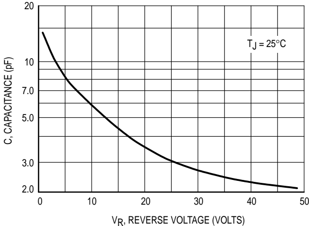
Figure 10. Typical Capacitance
