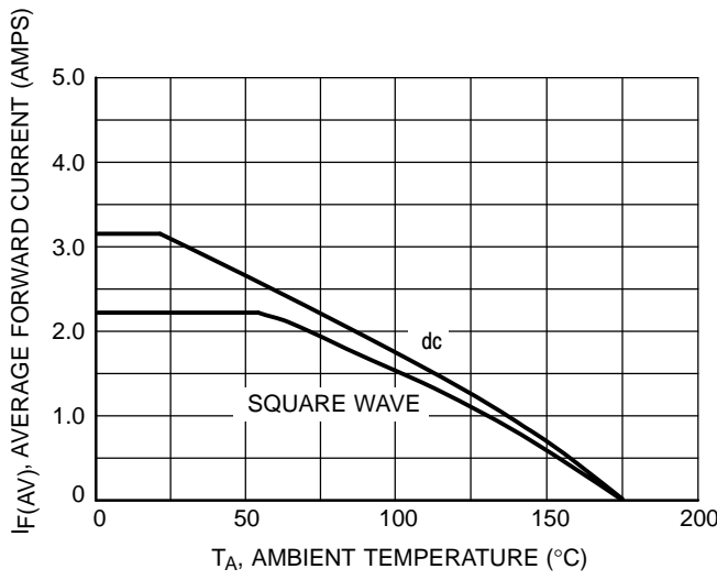
Figure 5. Current Derating
