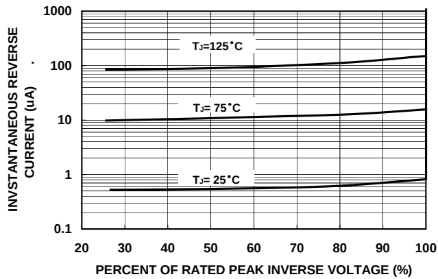
FIG. 3-TYPICAL REVERSE CHARACTERISTICS
