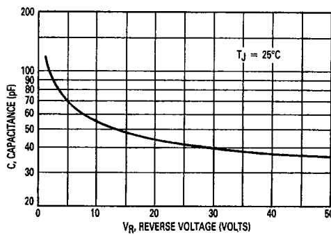
FIGURE 5 — TYPICAL CAPACITANCE
