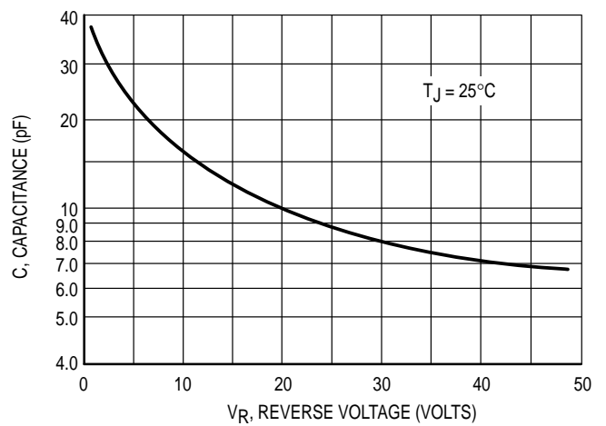
Figure 10. Typical Capacitance
