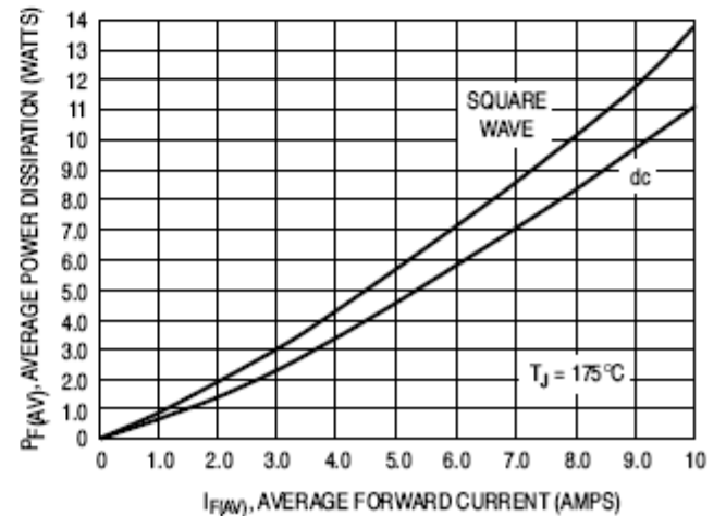
Figure 15. Power Dissipation
