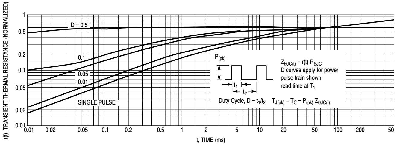
Figure 5. Thermal Response
