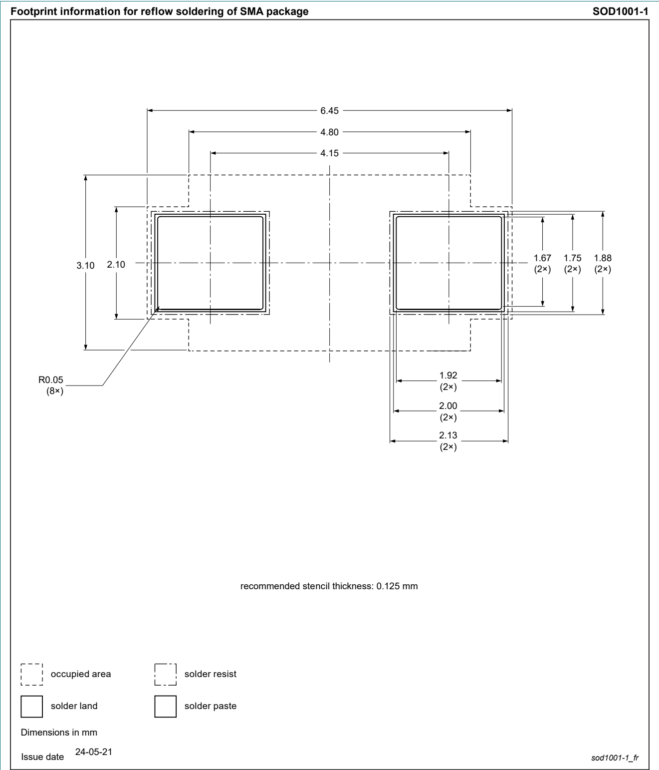
Fig. 14. Reflow soldering footprint for SMA (SOD1001-1)
