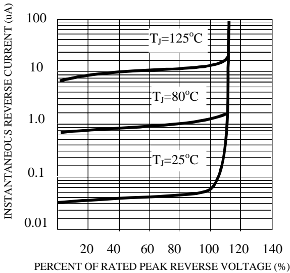
FIG. 3-TYPICAL REVERSE CHARACTERISTICS
