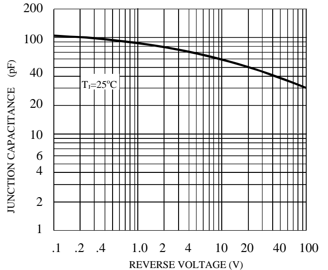
FIG. 6-TYPICAL JUNCTION CAPACITANCE
