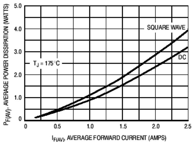
Figure 5. Power Dissipation
