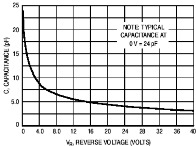
Figure 3. Typical Capacitance
