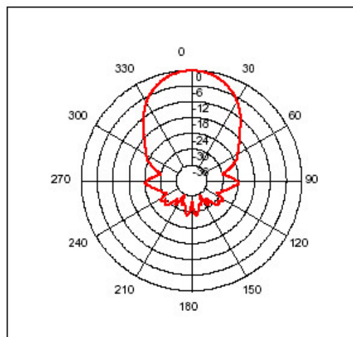
Beam Spread @ 40kHz (-6dB)
