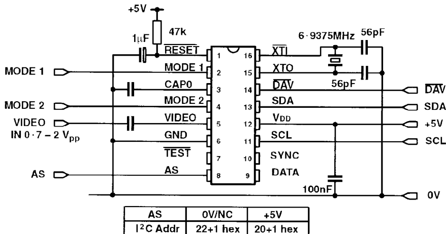
Fig. 3. Typical application diagram
