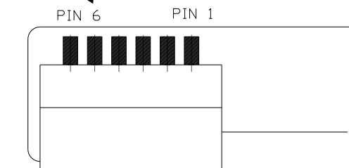
. Detailed Pin Define of LED Bar Connector
