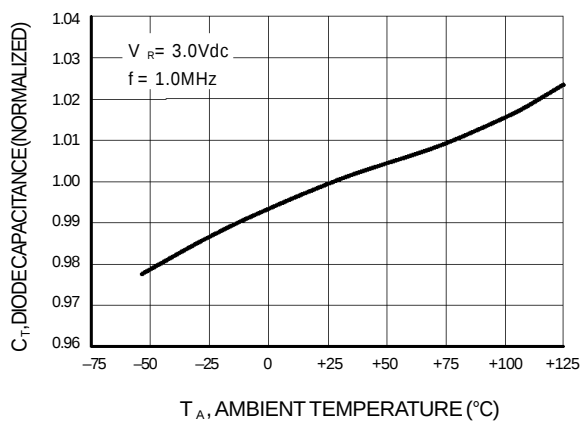
Figure 4. Diode Capacitance
