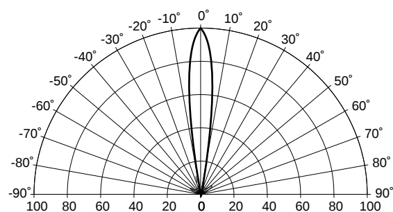
Fig. 4 Radiation Diagram
