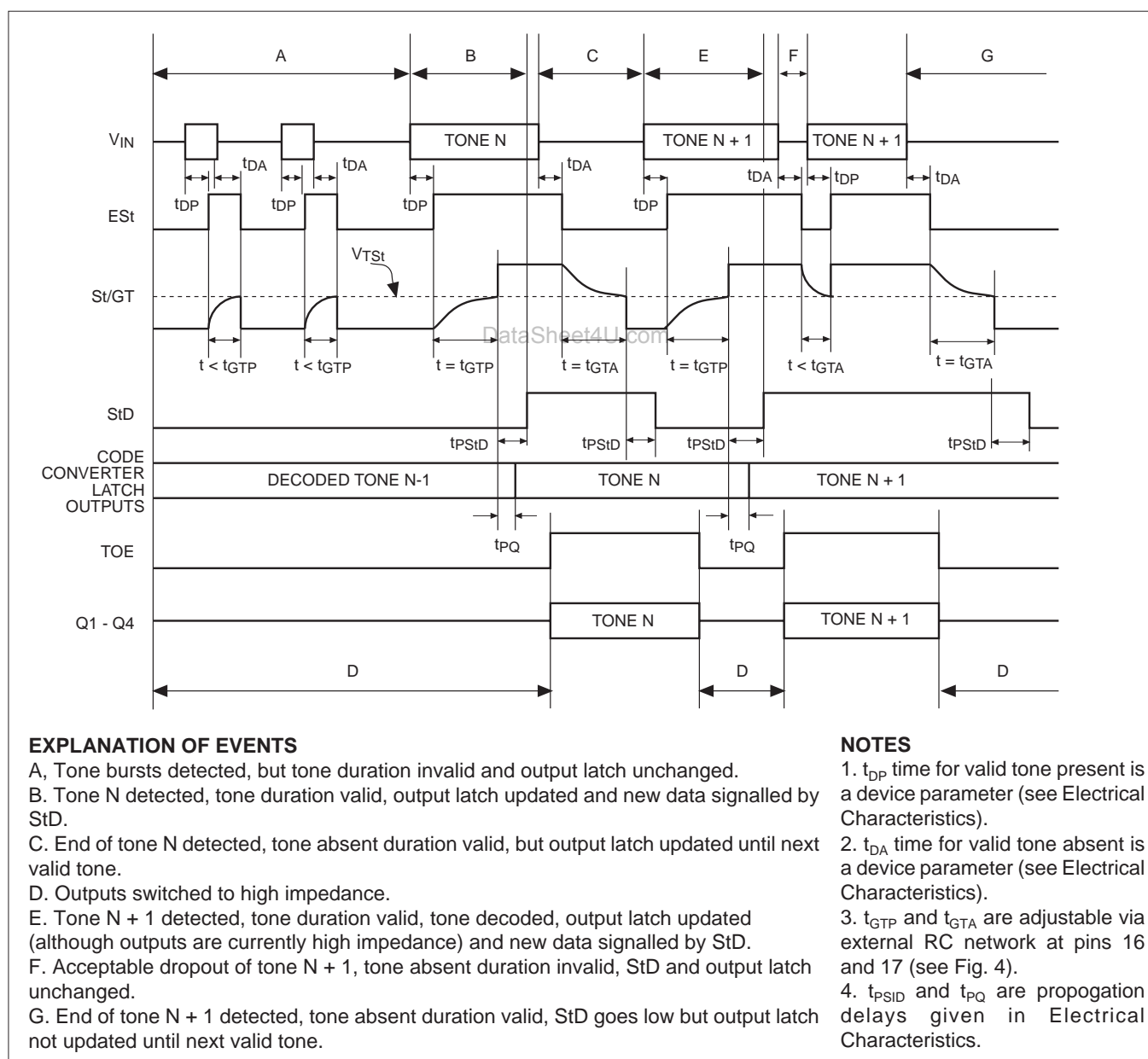
Figure 5: Timing diagram
