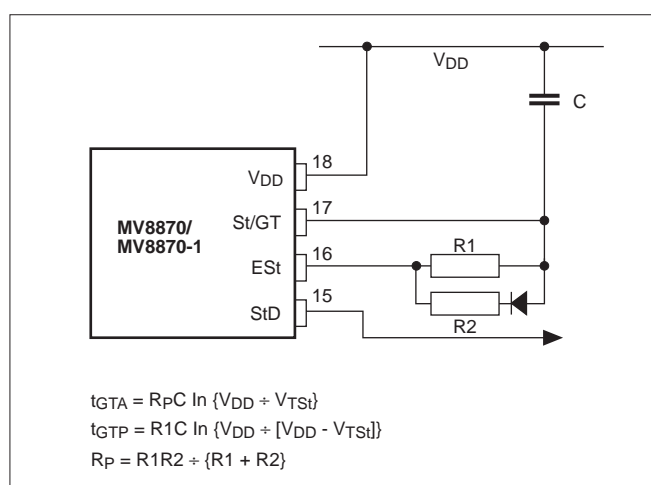
Figure 8b: Guard time adjustment ( t_{GTP} > t_{GTA} )
